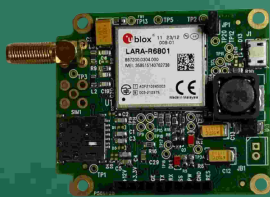
OMNI-U-BLOX-LARA-R6-LTE-Board
